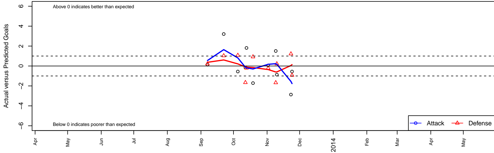
Impact SC B98 Dots are actual minus expected GF (blue circles) and GA (red triangles). Blue line is smoothed change in attack strength. Red is smoothed change in defense strength.
